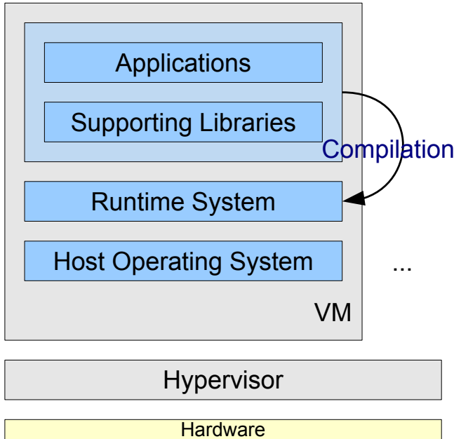
Figure 1. Software Stack
